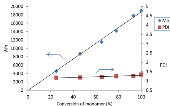
Figure 1. Pd(0)/ t -Bu 3 P-catalyzed Suzuki cross-coupling polymerization of 7-bromo-9,9-dihexylfluoren-2-ylboronic acid pinacol ester with PhPd( t -Bu 3 P)I as the initiator ([monomer] 0 = 15.4 mmol/L, [PhPd( t -Bu 3 P)I] 0 = 0.46 mmol/L, 2 M K 3 PO 4 (aq), THF, 0 °C; see the SI for details).
