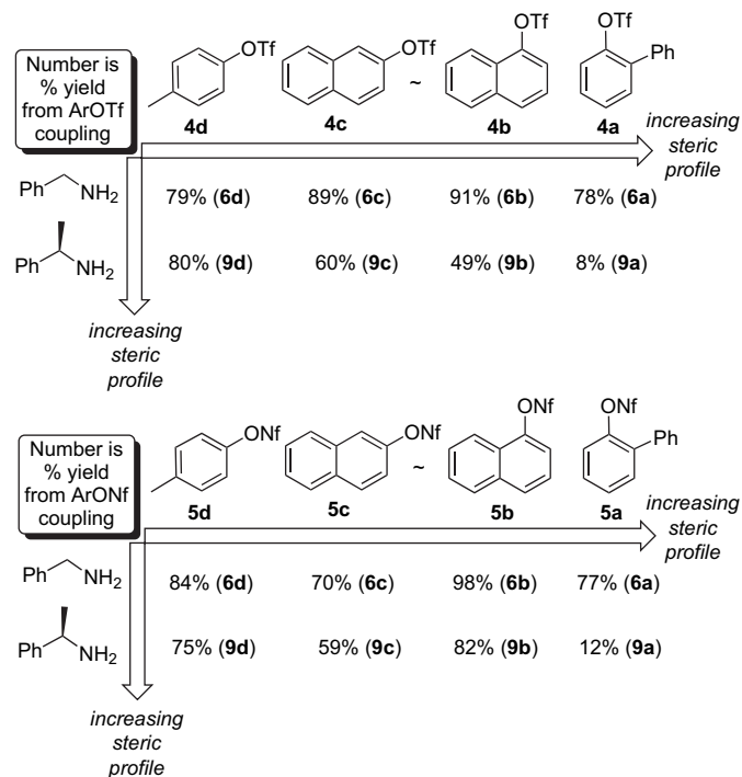
Scheme 2. Isolated chemical yields of C–N coupling products resulting from \text{Pd/X-Phos} 1a / \text{K}_3\text{PO}_4 catalysis of aryl triflates and nonaflates (identical conditions to Table 1; product shown in parentheses).
