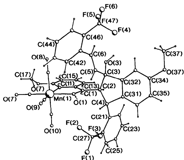
Fig. 1. Structure of [2-(1S^*,2R^*,3S^*) -1-hydroxy-1-(( E )-2-(2-trifluoromethylphenyl)ethenyl)-3-(2-trifluoromethylphenyl)-6-methoxy-2-indanylcabonyl- \kappa O )-6-methoxyphenyl- \kappa C^1 ]tetracarbonylmanganese ( 7a ), formed during cyclomanganation of 1-(3-methoxyphenyl)-3-(2-trifluoromethylphenyl)prop-2-en-1-one. Selected bond parameters: Mn-C(11) , 2.043(7) Å; Mn-O(1) , 2.052(5) Å; C(1)-O(1) , 1.251(8) Å, C(11)-Mn-O(1) , 79.0°. Other bond lengths and angles fall within expected ranges.
