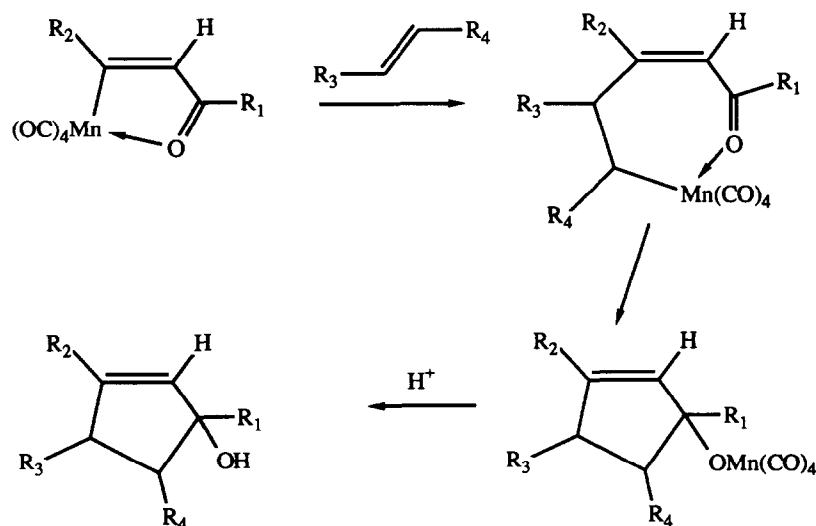
Scheme 3. Possible route from alkene-manganated chalcones and alkenes to cyclopentenol products 8 ( \text{R}_1 = 4-bromophenyl; \text{R}_2 = \text{R}_3 = 4-trifluoromethylphenyl; \text{R}_4 = 4-bromobenzoyl) and 12 ( \text{R}_1 = 4-chlorophenyl; \text{R}_2 = 3,4,5-trimethoxyphenyl; \text{R}_3 = H; \text{R}_4 = \text{COCH}_3 ).
