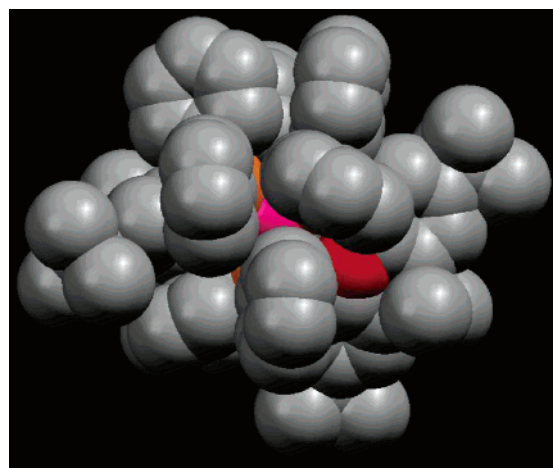
Figure 7. Space-filling model of \text{Pd}(4,7\text{-di-}t\text{-butylXantphos})_2 . Gray = carbon, red = oxygen, orange = phosphorus, and pink = palladium.
