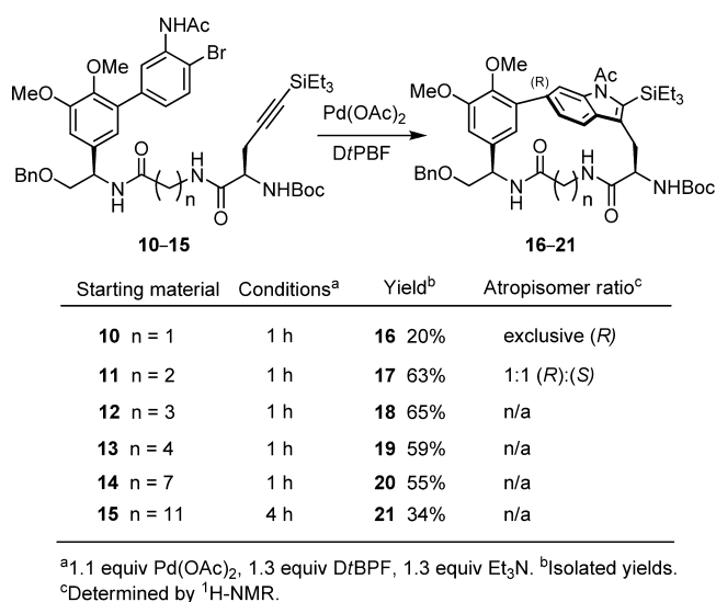
Figure 5. Cyclic peptide macrocyclizations.
