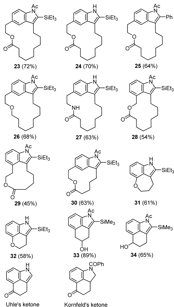
Figure 8. Scope of catalytic macrocyclization and cyclization reaction.
