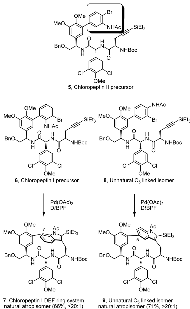
Figure 3. Additional isomeric macrocyclization substrates.
