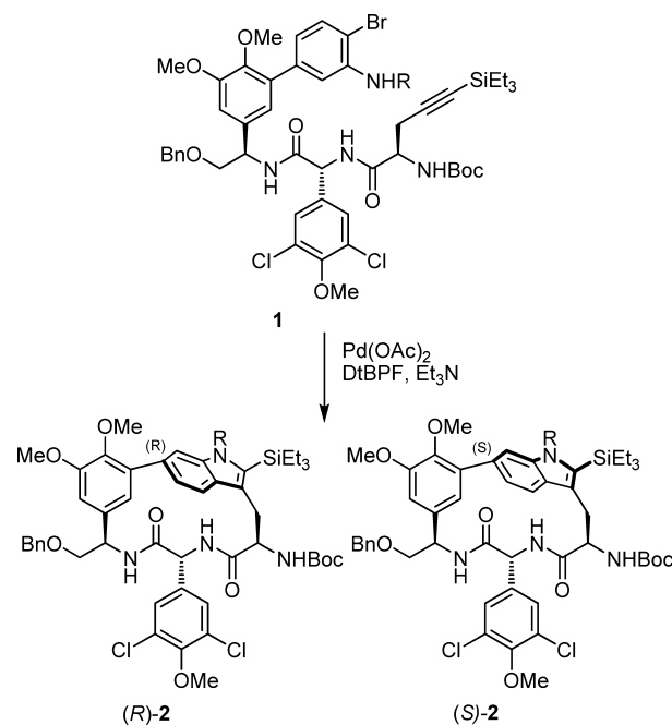
Figure 1. First-generation Pd(0)-mediated macrocyclization.
