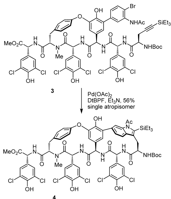
Figure 2. Second-generation macrocyclization.
