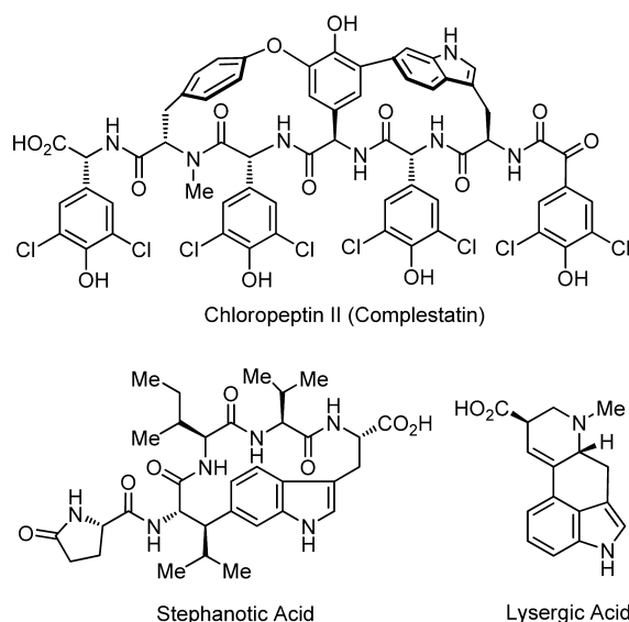
Figure 9. Key natural products containing macrocyclic and cyclic indoles.
