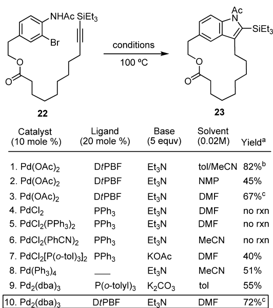
Figure 7. Optimization of catalytic Pd(0)-mediated macrocyclization.
