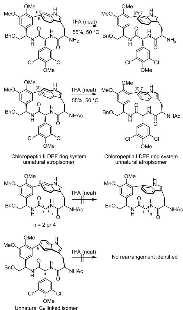
Figure 6. Acid-catalyzed rearrangement studies.
