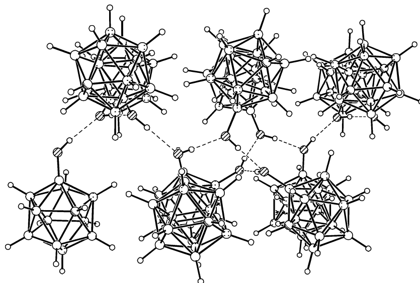
Figure 6. Double layers in the structure 5 (average H-bond parameters: O(2A)–H(2A) 0.82(2) Å, distances O(2A)···O(2B) and H(2A)···O(2B) 2.617 and 1.81 Å, respectively, O(2A)–H(2A)···O(2B) bond angle 170.2°).
