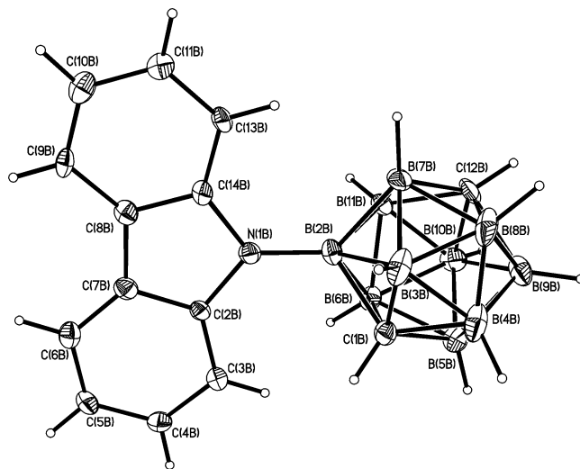
Figure 1. Molecular structure of one of the independent molecules (B) of N -(1,12-dicarba- closo -dodecaboran-2-yl)carbazole (1) (50% probability thermal ellipsoids). Selected bond distances (Å) for A[B] molecules: N(1)–B(2) 1.481(5) [1.472(5)], C(1)–B(2) 1.743(6) [1.725(6)], C(1)–B(3) 1.745(5) [1.655(6)], C(1)–B(4) 1.747(6) [1.677(6)], C(1)–B(5) 1.673(8) [1.691(6)], C(1)–B(6) 1.660(8) [1.719(6)], C(12)–B(7) 1.687(6) [1.651(7)], C(12)–B(8) 1.704(6) [1.718(9)], C(12)–B(9) 1.704(6) [1.705(7)], C(12)–B(10) 1.659(7) [1.659(6)], C(12)–B(11) 1.713(6) [1.648(7)]. Bond angle C(2)–N(1)–C(14): 105.0(5)° [107.5(5)°].
