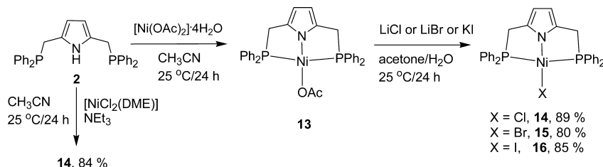
Scheme 4. Synthesis of Ni(II) Complexes 13–16 Bearing the PNP Pincer Ligand 2
