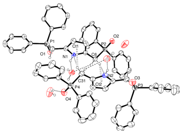
Figure 2. ORTEP diagram of (6\cdot2\text{H}_2\text{O})_2 with 30% probability ellipsoids. Most H atoms are omitted for clarity. Selected bond lengths (Å) and angles (deg): O1–P1 1.493(3), O3–P3 1.483(3), O4–P4 1.486(3), C1–P1 1.814(4), C25–P1 1.802(4), C2–N1 1.375(5), C2–C1–P1 115.2(3), O1–P1–C25 112.11(19), C25–P1–C1 105.26(19), C19–P1–C25 107.92(19), N1–C2–C1 122.4(4), C6 \cdots N2 3.574, H6b \cdots N2 2.674, C6–H6b \cdots N2 154.60; C31 \cdots N1 3.684, H31a \cdots N1 2.789, C31–H31a \cdots N1 153.82.
