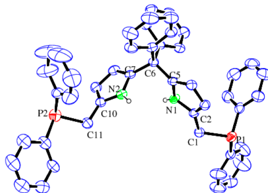
Figure 1. ORTEP diagram of 1,9-bis(diphenylphosphinomethyl)-diphenyldipyrrolylmethane, 5 (30% thermal ellipsoids). All hydrogen atoms except the pyrrolic NH are omitted for clarity. Selected bond lengths (Å) and angles (deg): P1–C1 1.846(6), C1–C2 1.501(7), C2–N1 1.368(7), C5–C6 1.521(8), P1–C1–C2 112.6(4), C5–C6–C7 111.6(5).
