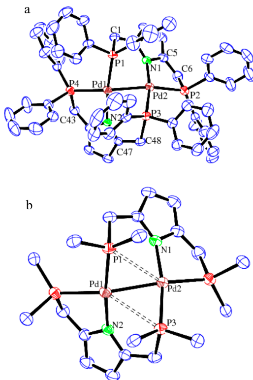
Figure 4. ORTEP diagram of \mathbf{12} \cdot 0.5(\text{C}_6\text{H}_6) with 30% probability ellipsoids: view b is showing the existence of the weak interactions between the diagonally positioned P and Pd atoms. All H atoms, the lattice benzene molecule, and the phenyl carbon atoms except the ipso carbons (view b) are omitted for clarity. Selected bond lengths (Å) and angles (deg): Pd1–Pd2 2.5470(5), N1–Pd2 2.111(4), N2–Pd1 2.090(4), P1–Pd1 2.2395(13), P2–Pd2 2.3504(14), P3–Pd2 2.2329(13), P3–Pd1 2.9744(14), P4–Pd1 2.3559(14), N2–Pd1–P1 171.32(11), N2–Pd1–P4 81.26(11), P1–Pd1–P4 104.09(5), N2–Pd1–Pd2 92.58(10), P1–Pd1–Pd2 79.84(4), P4–Pd1–Pd2 156.85(4), N2–Pd1–P3 72.26(11), P1–Pd1–P3 104.85(4), P4–Pd1–P3 146.67(4), Pd2–Pd1–P3 46.92(3), N1–Pd2–P3 169.58(11), N1–Pd2–P2 82.79(12), P3–Pd2–P2 106.38(5), N1–Pd2–Pd1 93.03(11), P3–Pd2–Pd1 76.65(4), P2–Pd2–Pd1 159.44(4).
