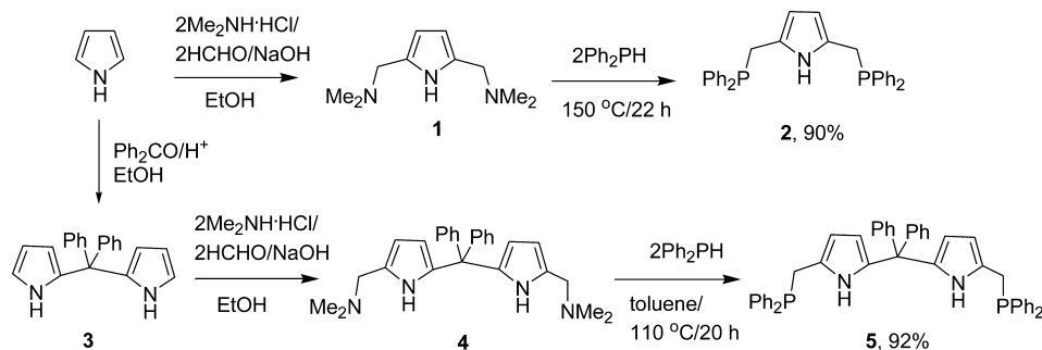
Scheme 1. Synthesis of the Pyrrole-Based PNP Pincer (2) and PNNP Type (5) Diphosphines
