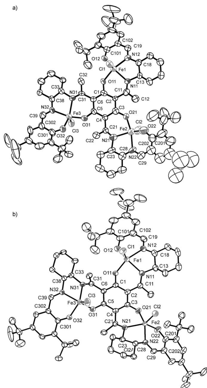
Figure 2. Molecular structures of the trinuclear complexes a) 3 rac and b) 3 RR ; thermal ellipsoids are drawn at the 50% probability level; hydrogen atoms are omitted for clarity.
