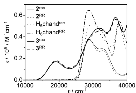
Figure 6. Electronic absorption spectra of 2 rac , 2 RR , H 6 chand rac , H 6 chand RR , 3 rac , and 3 RR measured at ambient temperatures in CH 2 Cl 2 .
