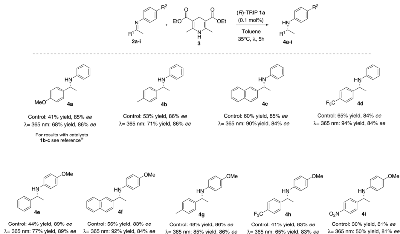
Figure 4. Effect of light on the asymmetric hydrogenation: screening of imines 2a-i . All reactions were carried out employing imine 2a-i (0.36 mmols, 1 eq), Hantzsch ester 3 (1.4 eq) and ( R )-TRIP 1a (0.01 eq) in 4.4 mL toluene under continuous illumination with a 365 nm LED lamp for 5 hours at 35°C. The control reactions were run in the same conditions without LED illumination. Isolated yield after chromatography are shown. The ee values were determined by HPLC on chiral stationary phase; changes on ee are within the experimental error.
