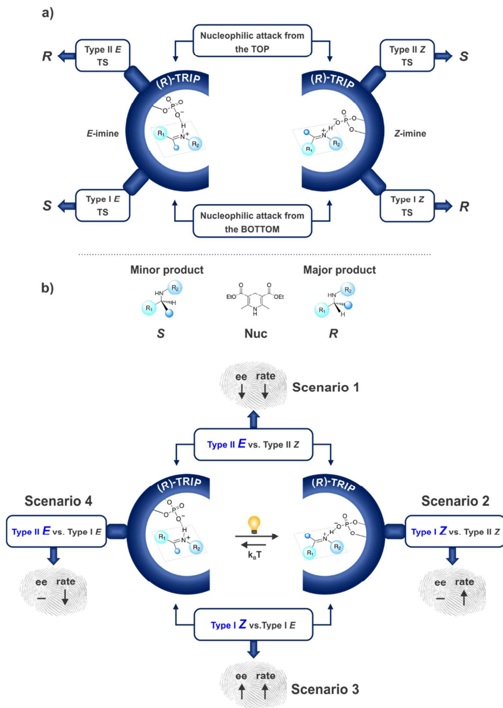
Figure 2. Transition states and produced fingerprint pattern upon photoisomerization for phosphoric acids catalyzed addition of nucleophiles to imines: a) Transition states proposed for the transfer hydrogenation of imines in the presence of Hantzsch ester analogue to Goodman's. 14 The example shows that four pathways (Type I Z, Type I E, Type II Z, Type II E) lead to different enantiomers depending on the imine configuration ( E or Z -imine) and on the nucleophilic attack site (top or bottom). R and S refer to the stereogenic center configuration in the product. b) Changes in characteristic fingerprint pattern (rate and enantiomeric excess ( ee )) upon illumination given the competition of two transition states. In case the major enantiomer is R only 4 out of 8 transition state combinations can be active (the transition states labelled in blue correspond to the major pathway in operation in case of ( R )-configured major product; for a complete set of scenarios see the SI). ↑, increase in ee or reaction rate; ↓ decrease in ee or reaction rate; — no change in ee ; ( R )-TRIP 1a (( R )-3,3'-Bis(2,4,6-triisopropylphenyl)-1,1'-binaphthyl-2,2'-diyl hydrogenphosphate).
