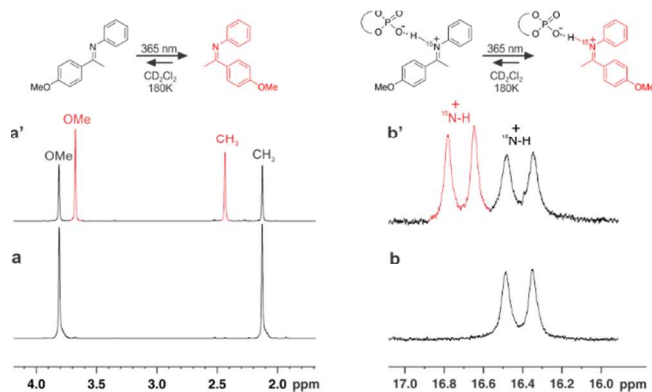
Figure 3. In situ NMR photoinduced isomerization of model imine 2a and its TRIP-complexes. a) The Me- and OMe- sections of 1 H-NMR spectra of imine 2a in CD 2 Cl 2 at 180 K (600 MHz) in the dark and after 90 min illumination (photostationary state) show the effective isomerization from E to Z of free imine 2a ; b) Low field sections of 1 H-NMR spectra of an imine 2a /( R )-TRIP 1a binary complex in CD 2 Cl 2 at 180 K (600 MHz) showing the characteristic signals of the 15 N-H in the hydrogen bond in the dark and after 90 min illumination (photostationary state). The spectra clearly shows that the imine photoisomerization is also possible inside the binary complex.
