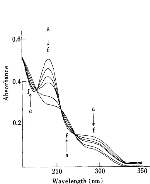
Fig. 1. UV Spectral Changes of Flutazolum (IF, 2.00 \times 10^{-5} M) with Time at pH 1.2 and 25^\circ\text{C}
