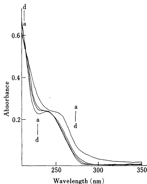
Fig. 2. UV Spectral Changes of Flutazolum (IF, 2.00 \times 10^{-5} M) and Its Hydrolyzate (IIIF, 2.00 \times 10^{-5} M) with Time at pH 7.4 and 25^\circ\text{C}
