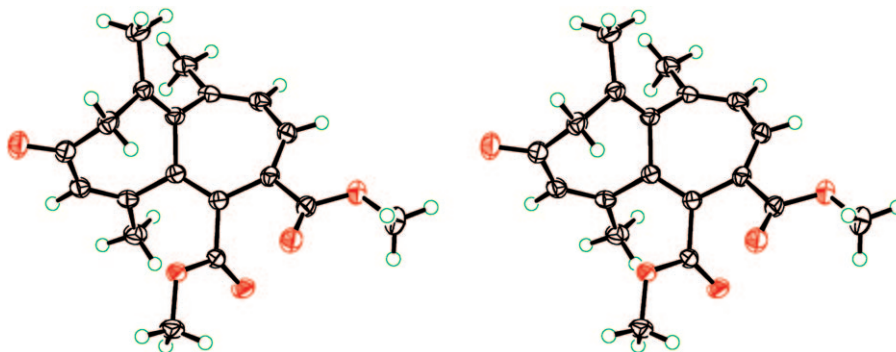
Fig. 1. Stereoscopic view of dimethyl 8,9-dihydro-1,6,10-trimethyl-8-oxoheptalene-4,5-dicarboxylate 4) ( 13 ) (50% probability ellipsoids)
