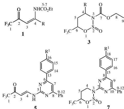
Figure 1. atom numbering for the NMR assignment of compounds 1 , 3 , 5 , and 7 .
