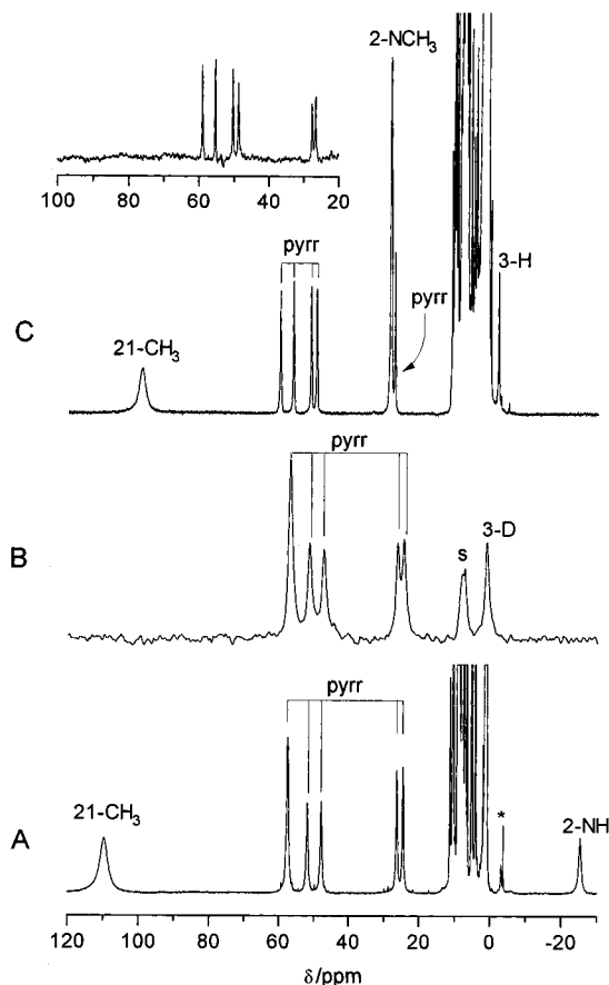
Figure 7. NMR spectra of paramagnetic mono- and dimethylated nickel(II) carbaporphyrin: (A) (2-NH-21-CH 3 CTPP)Ni II Cl (1H NMR, CDCl 3 , 293 K); (B) (2-NH-21-CH 3 CTPP- d 7 )Ni II Cl (2H NMR, CHCl 3 , 293 K); (C) (2-NCd 3 -21-CH 3 CTPP)Ni II Cl; inset (2-NCd 3 -21-CD 3 -CTPP)Ni II Cl (1H NMR, CDCl 3 , 293 K). Peak labels follow systematic numbering of the porphyrin ring or denote proton groups: pyr, regular pyrrole ring protons; s, solvent. Asterisk marks traces of diamagnetic (21-CH 3 CTPP)Ni II found due to some 2-NH proton dissociation in solution.
