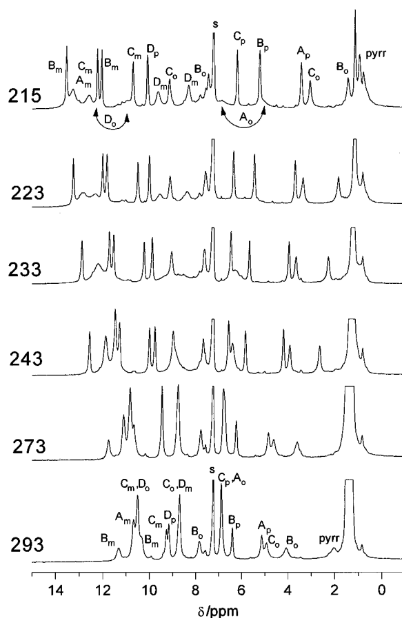
Figure 8. ^1\text{H} NMR spectra of the meso -phenyl region of (2\text{-NH-}21\text{-CH}_3\text{CTPP})\text{Ni}^{\text{II}}\text{Cl} in \text{CDCl}_3 at various temperatures. Peak labels denote respective ortho , meta , or para protons of unequivalent phenyl rings; s, solvent.
