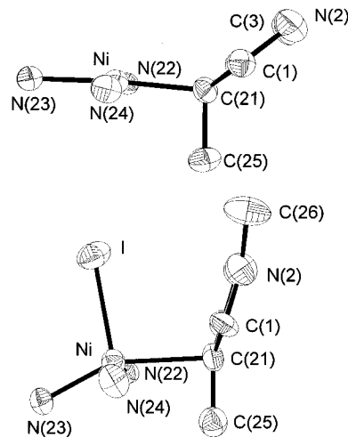
Figure 6. Comparison of nickel and C(21) environment geometry in (21\text{-CH}_3\text{CTPP})\text{Ni}^{\text{II}} (upper drawing) and (2\text{-NCH}_3\text{-}21\text{-CH}_3\text{CTPP})\text{Ni}^{\text{II}} (lower drawing).
