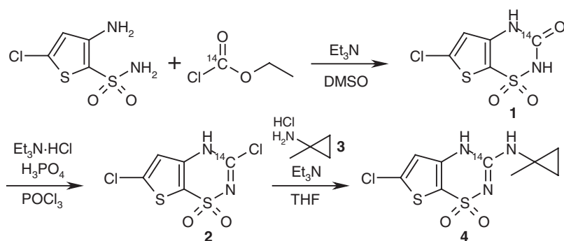
Scheme 1. Synthesis of [ ^{14}\text{C} ]NN414 ( 4 )
