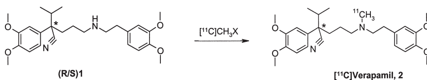
Figure 1. Synthesis of the enantiomers of [ ^{11}\text{C} ]verapamil (experimental details mentioned in Table 1)
