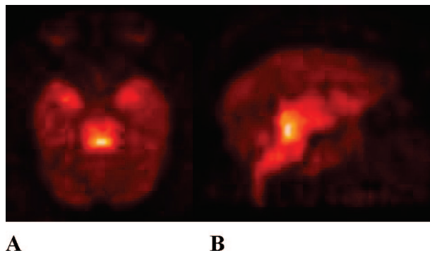
Figure 5. Summed (0–120 min) transaxial (A), and sagittal (B) images from microPET acquisitions in a male cynomolgus monkey after i.v. injection of 18.20 mCi of [ ^{11}\text{C} ]-( 37 ).
