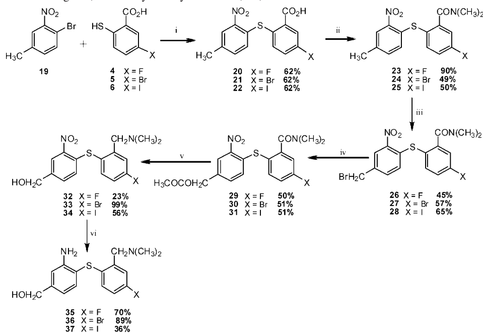
Scheme 3. Synthesis of the Target N,N -Dimethyl Benzylamines 35 , 36 , and 37 a
