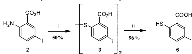
Figure 1. Substituted diaryl sulfide compounds.
