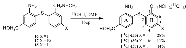
Scheme 4. Synthesis of [ 11 C]-( 35 ), [ 11 C]-( 36 ), and [ 11 C]-( 37 )
