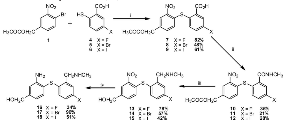
Scheme 2. Synthesis of the Monomethyl Precursors 16 , 17 , and 18 a
