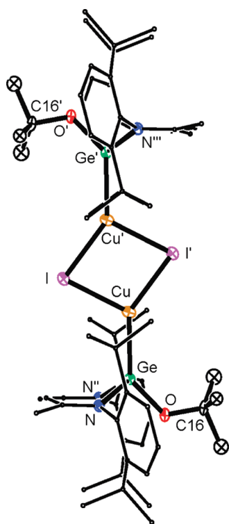
Figure 3. ORTEP diagram of \{\mu^1\text{-Cu}_2\text{I}_2\}[(\text{BDI})\text{GeO}^t\text{Bu}]_2 7 with H atoms omitted and BDI aryl group C atoms minimized for clarity; ellipsoid probability shown at 30%.
