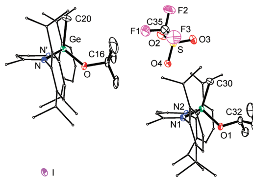
Figure 2. ORTEP diagrams of [(BDI)Ge(Me)O t Bu][I] 4 (left) and [(BDI)Ge(Me)O s Bu][OTf] 5b (right) with H atoms omitted and BDI aryl groups C atoms minimized for clarity; ellipsoid probability shown at 30%.
