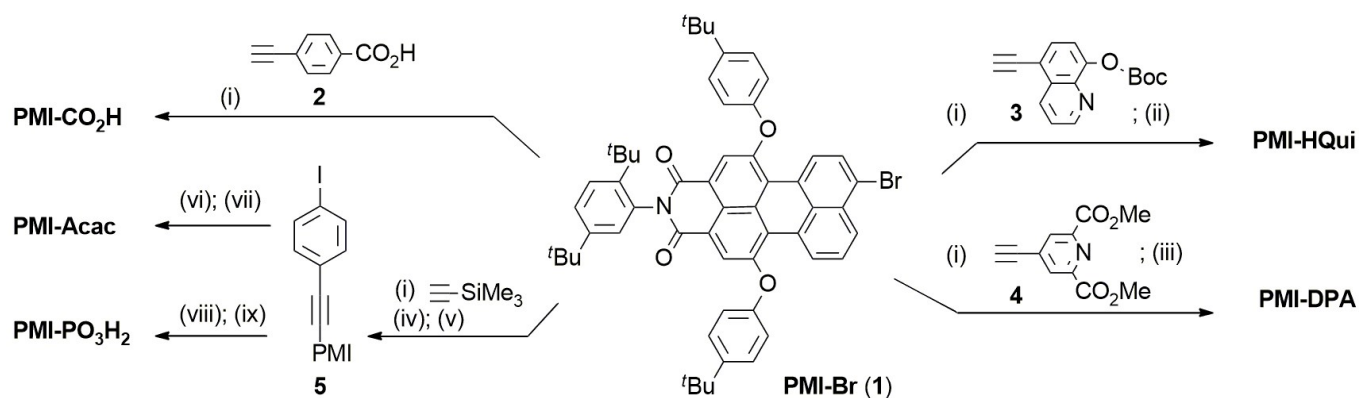
Scheme 1. Synthesis of the PMI dyes with different anchoring groups. (i) Pd(PPh 3 ) 4 , CuI, toluene, DIPEA or Et 3 N, [45 to 60] °C, [3 to 22] h; (ii) piperidine, DCM, r.t., 5 min; (iii) K 2 CO 3 , THF/H 2 O, 50 °C, 16 h; (iv) K 2 CO 3 , DCM/MeOH, r.t., 3 h; (v) 1,4-diiodobenzene, Pd(PPh 3 ) 4 , CuI, toluene, Et 3 N, 70 °C, 2 h; (vi) DMIBF, Pd(PPh 3 ) 4 , Cs 2 CO 3 , toluene/MeOH, 50 °C, 5 h; (vii) (a) Mo(CO) 6 , toluene/CH 3 CN/H 2 O, 90 °C, 3 h; (b) oxalic acid dihydrate, THF/H 2 O, 80 °C, 16 h; (viii) HPO 3 Et 2 , Et 3 N, Pd(PPh 3 ) 4 , THF, 60 °C, 24 h; (ix) (a) Me 3 Si-Br, Et 3 N, DCM, 50 °C, 5 h; (b) MeOH, r.t., 16 h. See ESI for synthesis and experimental details of compounds 3 and 4 .
