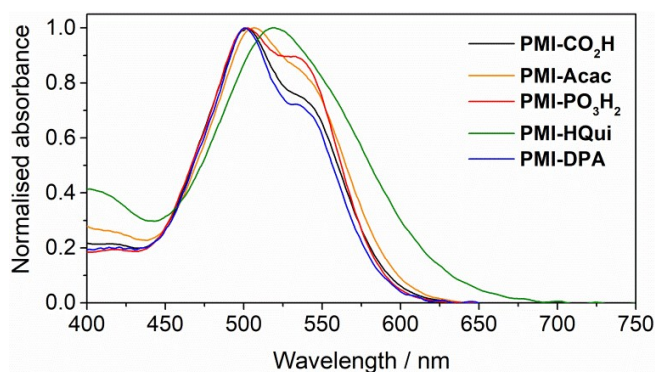
Figure 2. UV-Vis spectra of PMI dyes immobilised on a thin \text{TiO}_2 film (6 \mu\text{m} thickness) recorded at room temperature.
