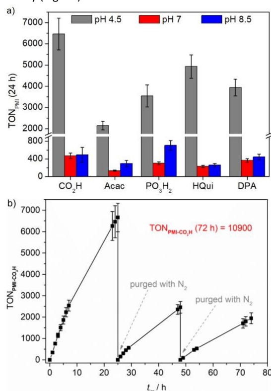
Figure 3. (a) Photocatalytic activity of PMI | \text{TiO}_2 | Pt expressed as \text{TON}_{\text{PMI}} after 24 h of irradiation in pH 4.5 AA (grey), pH 7 TEOA (red), and pH 8.5 TEOA (blue) solution (0.1 M each); (b) Long-term experiment ( \text{TON}_{\text{PMI-CO}_2\text{H}} vs t_{\text{irr}} ) using PMI-CO 2 H in pH 4.5 AA solution. Samples were purged with \text{N}_2 after 24 and 48 h. Conditions: UV-filtered simulated solar light irradiation (AM 1.5G, 100 \text{ mW cm}^{-2} , \lambda > 420 \text{ nm} ) of 1.25 mg PMI | \text{TiO}_2 | Pt in 3 mL ED (AA or TEOA) solution.
