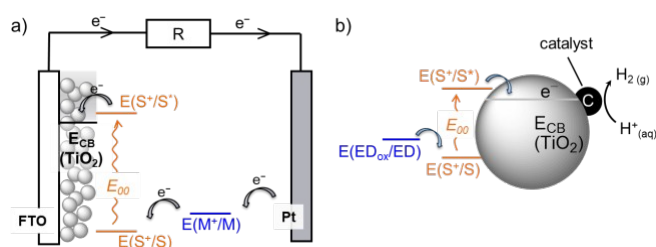
Figure 1. Schematic representation of solar energy conversion with dye-sensitised TiO 2 : (a) DSC 3 and (b) DSP systems 4 . See text for details.
