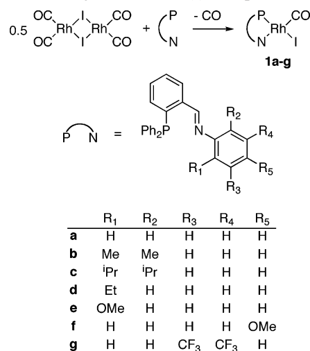
Scheme 2. Synthesis of Rh(I) Complexes 1a–g
