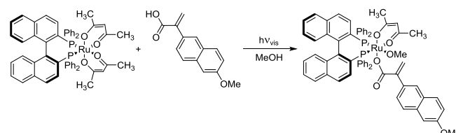
Scheme 1. Light activation of \text{Ru}(\text{acac})_2[(S)\text{-BINAP}] for the HY of alkenes.
