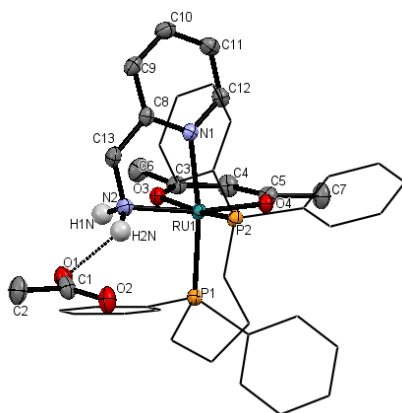
Figure 5. ORTEP-style drawing of 7 with ellipsoids at 50% probability level. All hydrogen atoms except H1N and H2N are omitted for clarity. Hydrogen atoms could not be located in the difference Fourier Maps and were calculated in ideal positions (riding model). For selected bond lengths and angles see Supporting Information.
