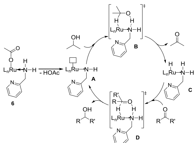
Scheme 4. Proposed catalytic cycle for ketone TH with 6 . L_n = dppb, acac.
