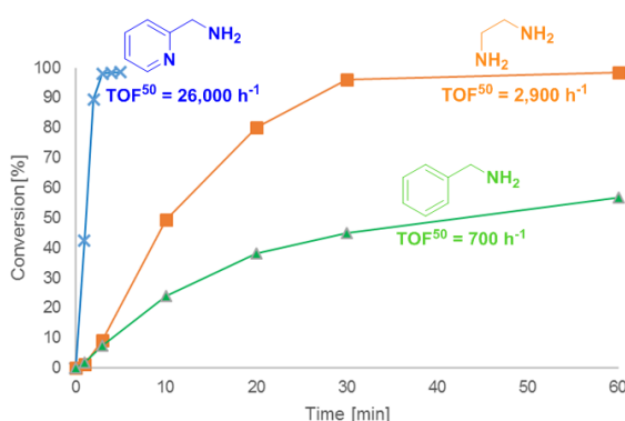
Figure 6. Transfer hydrogenation of acetophenone with complex 4 and 10 equiv. additives, ampy, en, bza. Conditions: t PrOH, 1 mmol a , 2 mol% NaO t Pr, 0.1 mol% 4 , 1.0 mol% additives, S/C/B = 100/0.1/2. x ampy, ■ en, ▲ bza.
