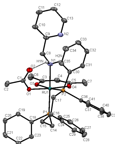
Figure 4. ORTEP-style drawing of 6 with ellipsoids at 50% probability level. All hydrogen atoms except H1N and H2N, and co-crystallized CH 2 Cl 2 are omitted for clarity. Hydrogen atoms could not be located in the difference Fourier Maps and were calculated in ideal positions (riding model). For selected bond lengths and angles see Supporting Information.
