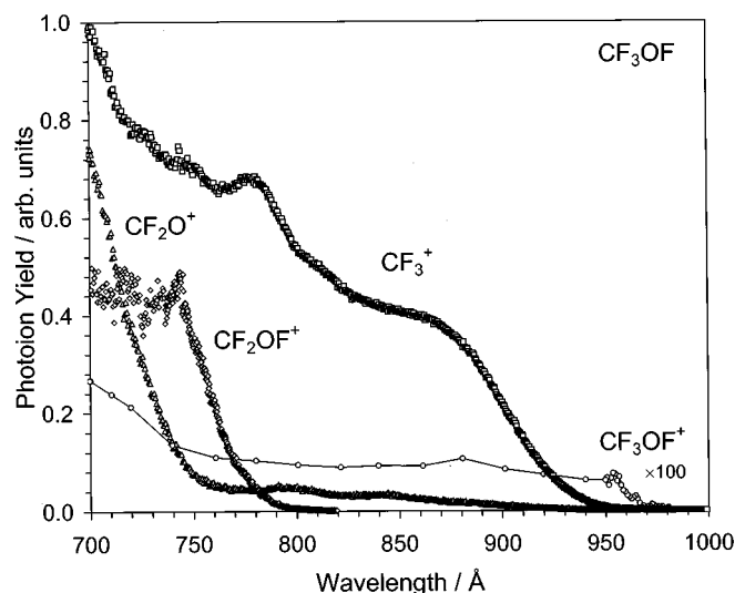
FIG. 5. An overview of the photoion yield curves of the parent \text{CF}_3\text{OF}^+ and its principal fragments, covering \sim 1000 – 700 Å. The relative abundances of various ions are correctly depicted in the figure, apart from quadrupole transmission factors. The parent \text{CF}_3\text{OF}^+ is very weak, but measurable. Discernible in the \text{CF}_2\text{O}^+ signal as two mild humps (at \sim 800 and \sim 845 Å) is a small contribution from parent ionization of the \text{CF}_2\text{O} precursor used in the synthesis of \text{CF}_3\text{OF} and present as a minor impurity. The \text{FCO}^+ curve is omitted from this figure, since it was completely attributable to fragmentation from this \text{CF}_2\text{O} impurity.
