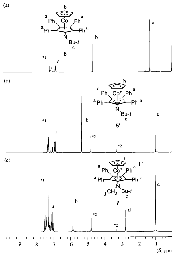
Fig. 1. ^1\text{H} -NMR spectra of 5 in \text{C}_6\text{D}_6 (a), 5' in \text{C}_6\text{D}_6 + \text{CD}_3\text{OD} (b), and 7 in \text{C}_6\text{D}_6 + \text{CD}_3\text{OD} (c) (*1: \text{C}_6\text{D}_6 , *2: \text{CD}_3\text{OD} ).
