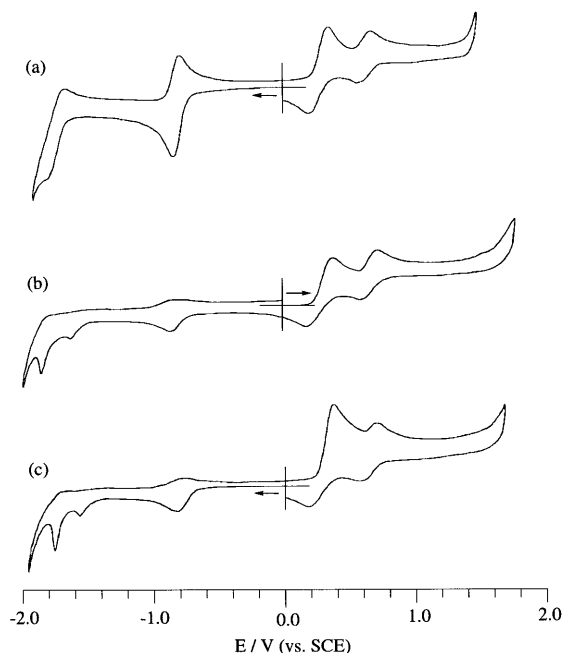
Fig. 5. CVs of 7 as a 1 mM–0.1 M \text{Bu}_4\text{NBF}_4\text{--CH}_3\text{CN} solution (a) and 3a as a precast film immersed in 0.1 M \text{Bu}_4\text{NBF}_4\text{--CH}_3\text{CN} measured on a Pt electrode (b and c) at the scan rate of 50 \text{ mVs}^{-1} .
