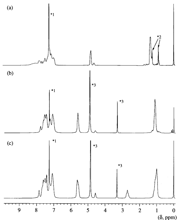
Fig. 3. ^1\text{H} -NMR spectra of 2a in \text{C}_6\text{D}_6 (a), 2a' in \text{C}_6\text{D}_6 + \text{CD}_3\text{OD} (b), and 3a in \text{C}_6\text{D}_6 + \text{CD}_3\text{OD} (c) (*1: \text{C}_6\text{D}_6 , *2: n -hexane, and *3: \text{CD}_3\text{OD} ).
