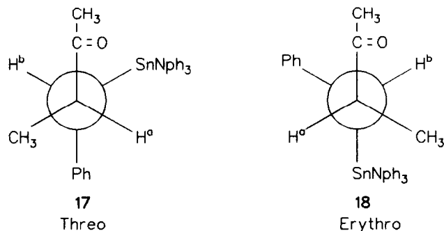
Fig. 2. Preferred conformations of threo and erythro 3-methyl-4-(trineophylstannyl)butan-2-ones ( 17 and 18 ) (only one isomer of each is shown).
