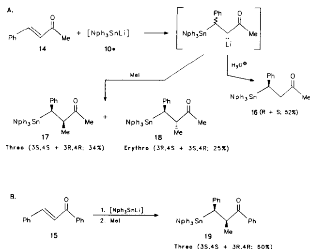
Fig. 1. Addition of trineophyltinlithium to: (A) benzylidenacetone; (B) chalcone.
