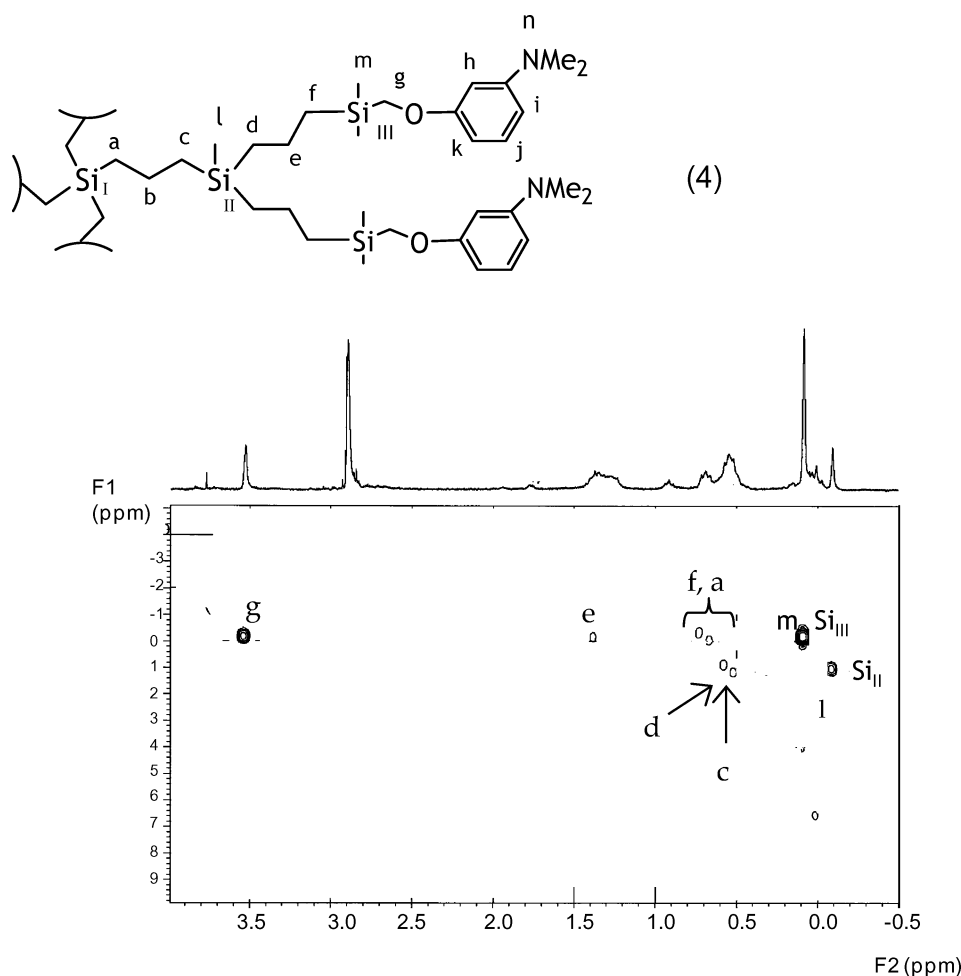
Fig. 2 2D\{^1H-^{29}Si\} -HMBC spectrum of dendrimer 4.
