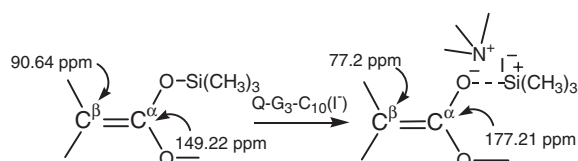
Figure 2. 13 C NMR shifts of the silyl acetal with quaternarized dendrimer Q-G 3 -C 10 (I − ).
