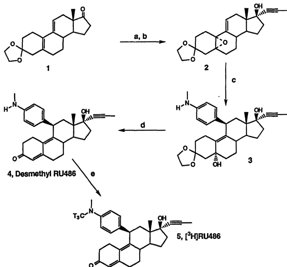
FIGURE 1. Synthetic route to [^3\text{H}] RU486. a, \text{H}_2\text{O}_2 ; b, \text{Me}-\text{C}\equiv\text{C}-\text{Li} ; c, 4-(trimethylsilyl methylamino)phenylmagnesium bromide; d, PTS, EtOH; e, \text{T}_3\text{CMeI} in DMF-toluene, 1:1, 72 hours at 70^\circ\text{C} .
