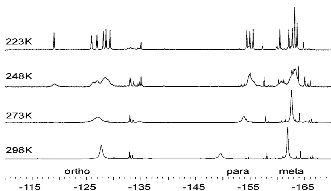
Figure 4. Dynamic ^{19}\text{F} NMR spectra of the \text{Mes}_2\text{PH} \cdot \text{B}(\text{C}_6\text{F}_5)_3 adduct 11 (in d_8 -toluene).
