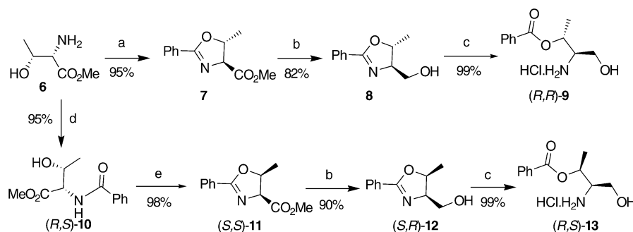
Scheme 3. Synthesis of the monoprotected aminodiols 9 and 13 : a) Ethyl benzimidate hydrochloride, Et 3 N, CH 2 Cl 2 , room temperature, 48 h; b) LiAlH 4 , Et 2 O, reflux; c) THF, 2M HCl, room temperature; d) benzoyl chloride, Et 3 N, CH 2 Cl 2 ; e) thionyl chloride, 0°C, 16 h.
