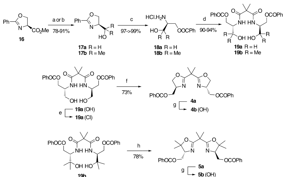
Scheme 5. Synthesis of BO 4 and 5 from L-serine: a) DIBAH, 17a ; b) \text{MeMgI} , \text{Et}_2\text{O} , reflux, 17b ; c) 2 M HCl, room temperature, 18a and 18b ; d) \text{Et}_3\text{N} , \text{ClCOC}(\text{Me})_2\text{COCl} , \text{CH}_2\text{Cl}_2 , 0 °C to room temperature, 19a and 19b ; e) \text{SOCl}_2 , reflux, 6 h; f) toluene, \text{Et}_3\text{N} , reflux; g) 1 % NaOH in methanol, room temperature; h) methanesulfonic acid, \text{CH}_2\text{Cl}_2 , reflux, see reference [10b].
