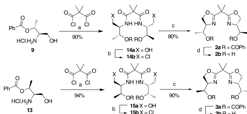
Scheme 4. Synthesis of BO ( R,R )- 2 and ( R,S )- 3 from the monoprotected aminodiols 9 and 13 : a) \text{Et}_3\text{N} , \text{CH}_2\text{Cl}_2 ; b) thionyl chloride, reflux, 6 h; c) toluene, \text{Et}_3\text{N} , reflux 6 or 16 h; d) 1 % sodium hydroxide in methanol, room temperature.
