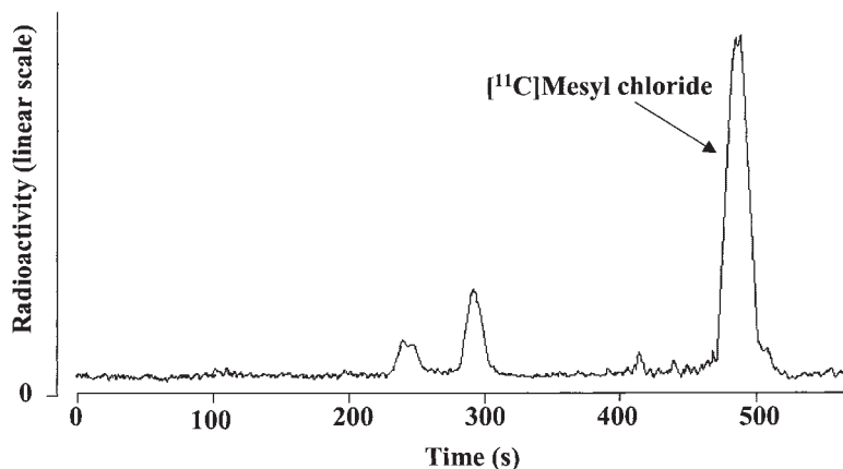
Figure 2. HPLC analysis (system A) of crude NCA [ 11 C]mesyl chloride produced by route 2
