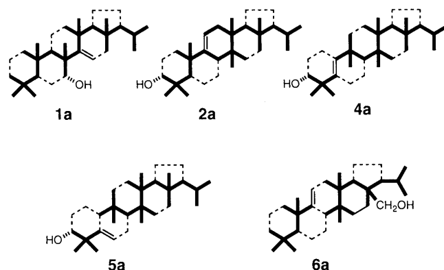
Fig. 1. Partial Structures of 1, 2, 4–6 Revealed by HMBC (Shown by Heavy Lines)
