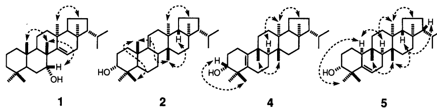
Fig. 2. NOEs Observed in the NOESY Spectra of 1, 2, 4 and 5
