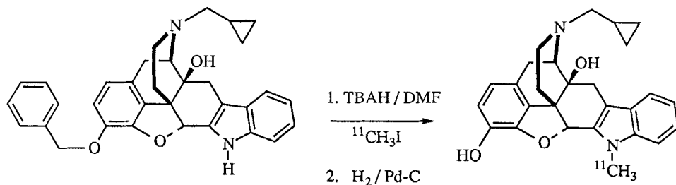
Scheme 2. Radiosynthesis of [ ^{11}\text{C} ]MeNTI.
