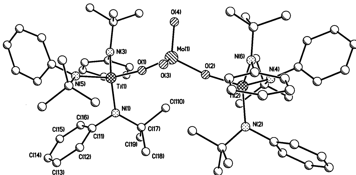
Figure 5. PLUTO drawing of the molecular structure of \text{O}_2\text{Mo}\{[\mu\text{-O}]\text{Ti}(\text{tBuNPh})_3\}_2 as determined by single-crystal X-ray diffraction. See Table 2 for selected bond lengths and angles.
