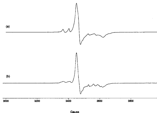
Figure 2. EPR spectrum (frozen toluene, 103 K) of (\text{tBuO})_3\text{Mo}[\mu\text{-N}]\text{Ti}(\text{NRAr})_3 (a) simulated with g_1 = 1.954 , g_2 = 1.944 , g_3 = 1.861 , a_1 = 30 , a_2 = 40 , a_3 = 16 G, (b) observed.
