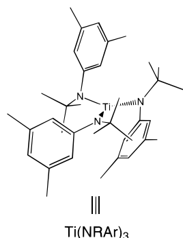
Figure 1. Line drawing of \text{Ti}(\text{NRAr})_3 based on the previously reported X-ray structure.
