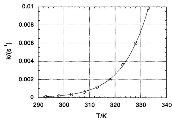
Figure 3. Exponential least-squares fit of first-order rate constants ( k ) versus temperature (K) to the Eyring equation k = (k_B T/h) \exp(-\Delta S^\ddagger/R) \exp(-\Delta H^\ddagger/RT) for the thermal conversion of (^t\text{BuO})_3\text{Mo}[\mu\text{-N}]\text{Ti}(\text{N}(\text{R}^i\text{Ar})_3)_3 to (^t\text{BuO})_2(\text{N})\text{Mo}[\mu\text{-O}]\text{Ti}(\text{N}(\text{R}^i\text{Ar})_3)_3 with tert -butyl radical loss (see Scheme 1). Activation parameters obtained from the fit are \Delta H^\ddagger = 21.4 \pm 0.2 \text{ kcal mol}^{-1} and \Delta S^\ddagger = -3.7 \pm 0.6 \text{ cal mol}^{-1} \text{ K}^{-1} .
