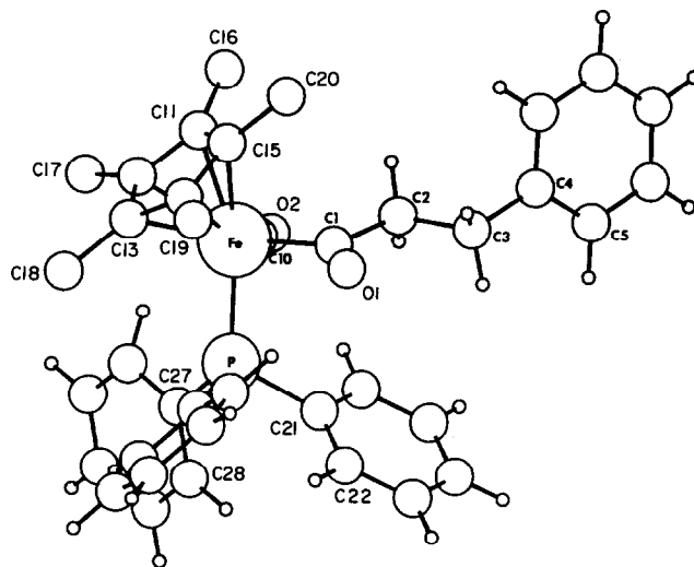
Fig. 1. Molecular structure of ( RS )-[( \eta^5 -C 5 Me 5 )Fe(CO)(PPh 3 )COCH 2 CH 2 Ph] ( 12 ).
