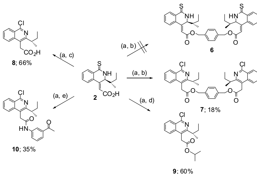
Scheme 2. Reagents and conditions: (a) SOCl 2 , CH 2 Cl 2 , 0 °C to rt, 0.5 h; (b) HOCH 2 -p-(C 6 H 4 )-CH 2 OH, CH 2 Cl 2 , rt, 1 h; (c) NaOH, 0.5 h; (d) Me 2 CHOH, CH 2 Cl 2 , rt, 1 h; (e) NH 2 -m-(C 6 H 4 )-COMe, Et 3 N, CH 2 Cl 2 , rt, overnight.
