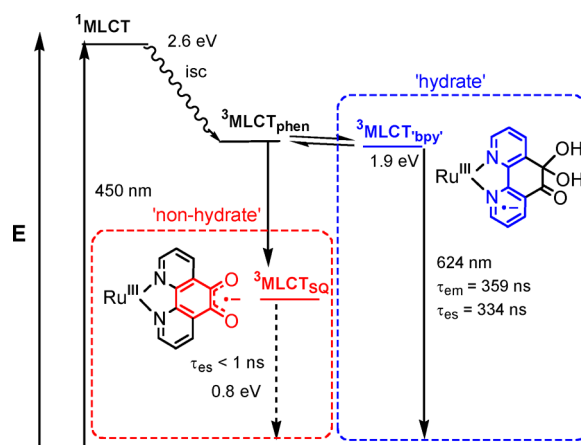
Figure 2. Proposed Jablonski diagram for \mathbf{1}^{2+} in MeCN (red box) or \mathbf{1H}_2\text{O}^{2+} in water (blue box). Deprotonation of \mathbf{1H}_2\text{O}^{2+} to \mathbf{1}(\text{OH})^+ shifts the emission maxima from 624 to 602 nm.
