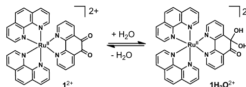
Scheme 1. Hydration Equilibrium for Complex 1^{2+} in Water
