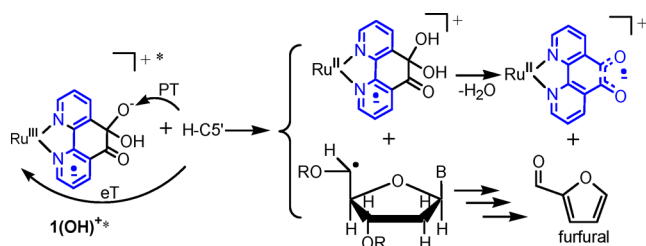
Scheme 2. Proposed PCET Mechanism between 1(\text{OH})^{2+} and DNA
