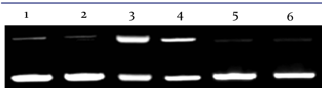
Figure 1. Ethidium bromide stained 1% agarose gel of photocleavage products of RuPD and pUC18: 1 \mu\text{g}/1\ \mu\text{L} , 0.154 mM pUC18 DNA base pairs (4 mM phosphate, 50 mM NaCl, pH = 7.4) and 27 \mu\text{M} of the chloride salt of the ruthenium complex, irradiated (when applicable) at 470 nm for 2 h; lane 1, plasmid only; lane 2, RuPD dark in presence of \text{O}_2 ; lane 3, RuPD irradiated in presence of \text{O}_2 ; lane 4, RuPD irradiated, deaerated; lane 5, [\text{Ru}(\text{phen})_3]^{2+} irradiated, deaerated; lane 6, [(\text{phen})_2\text{Ru}(\text{dppz})]^{2+} irradiated, deaerated.
