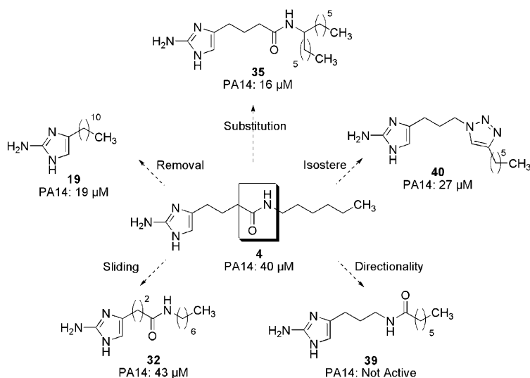
Scheme 8. PA14 inhibition IC_{50} values from selected SAR analogues.
