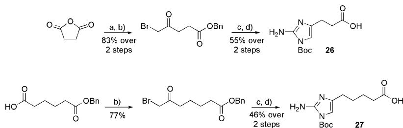
Scheme 4. Synthesis of Boc-2-AI linker acids: a) BnOH, TEA, DMAP, CH 2 Cl 2 (87%); b) i) (COCl) 2 , DMF (cat.), CH 2 Cl 2 ; ii) CH 2 N 2 , Et 2 O/CH 2 Cl 2 , 0 °C; iii) conc. HBr; c) Boc-guanidine, DMF; d) H 2 (1 atm), 10% Pd/C, THF, DMAP: 4-dimethylaminopyridine; TEA: triethylamine.
