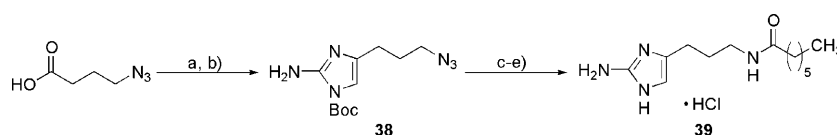
Scheme 7. A native amide bond approach: a) i) (\text{COCl})_2 , DMF (cat.), \text{CH}_2\text{Cl}_2 ; ii) \text{CH}_3\text{N}_2 , \text{Et}_2\text{O}/\text{CH}_2\text{Cl}_2 , 0^\circ\text{C} ; iii) conc. HBr (90%); b) Boc-guanidine, DMF (63%); c) i) \text{H}_2 (1 atm), 10% Pd/C, THF; ii) heptanoic anhydride (70%); d) TFA, \text{CH}_2\text{Cl}_2 ; e) 2 M HCl/ \text{Et}_2\text{O} (99%).
