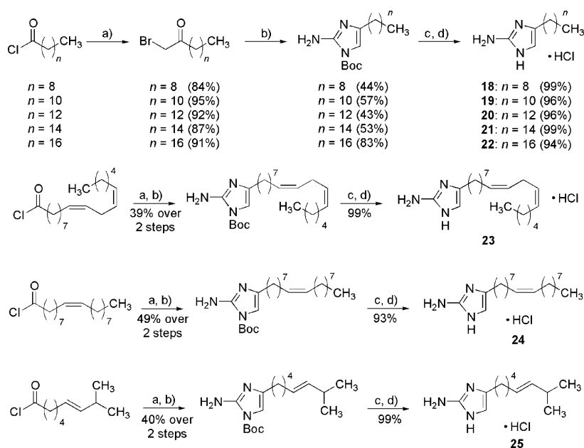
Scheme 3. Deletion of the amide bond: a) i) CH 2 N 2 , Et 2 O/CH 2 Cl 2 , 0°C; ii) conc. HBr; b) Boc-guanidine, NaI, DMF; c) TFA, CH 2 Cl 2 ; d) 2 M HCl/Et 2 O. Boc: tert -butoxycarbonyl; TFA: trifluoroacetic acid.
