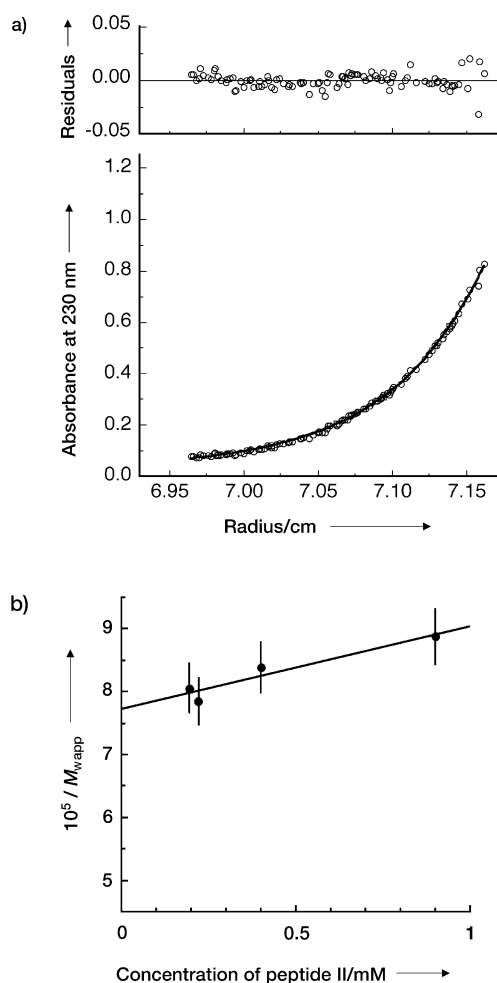
Figure 6. a) Sedimentation equilibrium analysis of peptide II. Peptide II (195 \mu M) was run at 40000 rpm at 20°C in 1 mM sodium citrate, 1 mM sodium borate, 1 mM sodium phosphate, and 10 mM sodium chloride (pH 7.3). b) Relationship between the peptide concentration and observed molecular weight ( M_{app} ). The mean molecular weight ( M_w ), which corresponds to the reciprocal of the intercept on the ordinate at zero concentration, was calculated as (1.30 \pm 0.065) \times 10^4 , which suggests that peptide II exists as a hexamer in the given solution.
