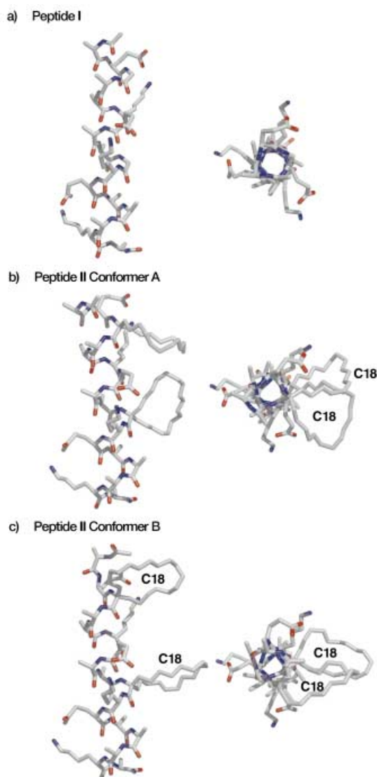
Figure 3. Energy-minimized \alpha -helical structures of a) peptide I (original Baldwin peptide), b) conformer A of peptide II, c) conformer B of peptide II. Conformers A and B differ in the orientations of the two 18-membered rings. Conformer A is more stable than conformer B. Water was used as a solvent in the force field calculations.
