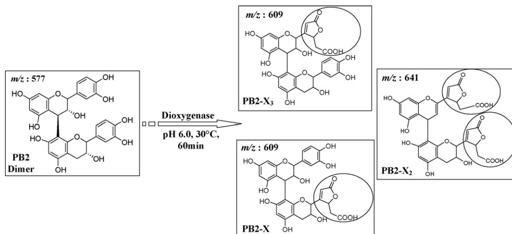
Fig. 5. The proposed dioxygenase reaction mechanism on PB2 & resulting oxidized products.
