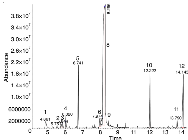
Fig. 1. TI chromatogram of catalytic conversion products of geraniol on micro-mesoporous zeolite R-BEA-25 ( m_{\text{cat}}/m_{\text{geraniol}}=1/142 , reaction carried out under simultaneous microwave and ultrasound irradiation (MW/US, 550 W/300 W, in a argon atmosphere at 80 °C, run time: 1.5 h): (1) \beta -myrcene, \text{C}_{10}\text{H}_{16} , (2) pseudo-limonene, \text{C}_{10}\text{H}_{16} , (3) trans - \beta -ocymene, \text{C}_{10}\text{H}_{16} , (4) \beta -ocymene, \text{C}_{10}\text{H}_{16} , (5) \beta -linalool, \text{C}_{10}\text{H}_{18}\text{O} , (6) nerol, \text{C}_{10}\text{H}_{18}\text{O} , (7) cis -isogeraniol, \text{C}_{10}\text{H}_{18}\text{O} , (8) trans -geraniol, \text{C}_{10}\text{H}_{18}\text{O} , (9) isopulegol, \text{C}_{10}\text{H}_{18}\text{O} , (10) trans,trans -farnesol, (2 E ,6 E )-3,7,11-trimethyl-2,6,10-dodecatrien-1-ol, \text{C}_{15}\text{H}_{26}\text{O} , (11) succinic acid, di(neryl)ester, \text{C}_{24}\text{H}_{38}\text{O}_4 , (12) (2 E ,6 E )-6,11-dimethyl-2,6,10-dodecatrien-1-ol, \text{C}_{14}\text{H}_{24}\text{O}
