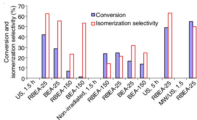
Fig. 6. Geraniol conversion under US (350 W, 1.5 and 5 h) and combined US/MW (300 W/550 W, 1.5 h) irradiation in the presence of micro- and micro-mesoporous beta-type zeolites. Effect of ultrasound irradiation time on degree of geraniol conversion and selectivity both to linalool and to nerol undividually; reaction conditions: catalyst loading – 0.92 mol of geraniol/g catalyst, argon atmosphere, run time 1.5 h, 5.0 h, temperature 80 °C
