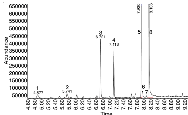
Fig. 2. TI Chromatogram of catalytic conversion products of geraniol on microporous zeolite BEA-25 ( m_{\text{cat}}/m_{\text{geraniol}} = 1/26.7 , reaction carried out under ultrasound irradiation (US, 200 W, solvent – 38.5 mL methanol, medium – air, temperature 30 °C, run time – 1 h). 1 – \beta -myrcene, C 10 H 16 , 2 – \beta -ocymene, C 10 H 16 , 3 – \beta -linalool, C 10 H 18 O, 4 – linalool, methyl ether, 5 – nerol, methyl ether, C 11 H 20 O, (2Z)-1-methoxy-3,7-dimethylocta-2,6-diene, 6 – nerol, C 10 H 18 O, 7 – cis -isogeraniol, C 10 H 18 O, 8 – trans -geraniol, C 10 H 18 O
