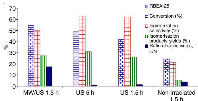
Fig. 8. Comparison of activities of different combined systems with micro-mesoporous zeolite RBEA-25 in the conversion of geraniol. Reaction conditions: catalyst loading – 0.92 mol of geraniol/g catalyst, argon atmosphere, run time – 1.5 h, 5.0 h, temperature – 80 °C, US (350 W), US/MW (300 W/550 W)
