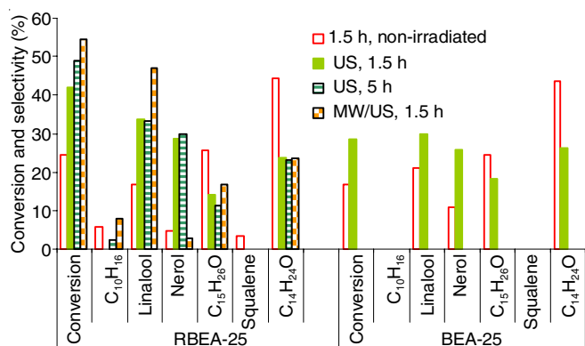
Fig. 5. Comparison of catalytic activities (at 80 °C, medium – Ar) of non-irradiated and irradiated zeolites with ultrasound (RBEA-25 and BEA-25) in reaction of geraniol conversion by • irradiation during 1.5 h, US power- 350 W, • irradiation during 5 h, • with combined US/MW irradiation during 1.5 h, US power - 300 W, MW power-550 W
