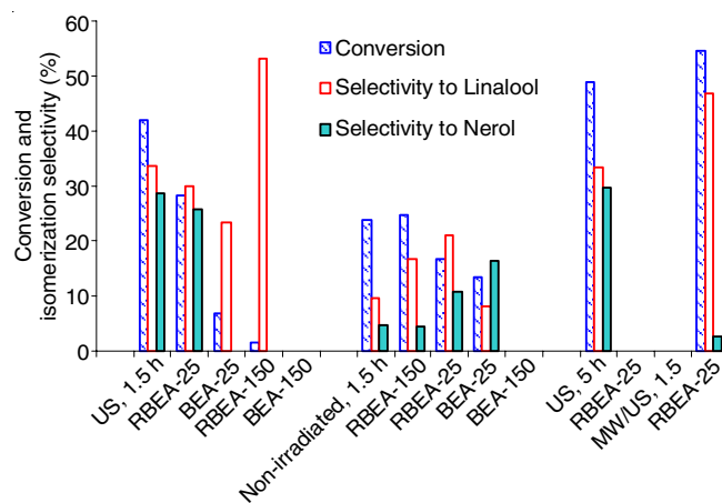
Fig. 7. Geraniol conversion under US (350 W) and combined US/MW (300 W/550 W) irradiations in the presence of micro- and micro-mesoporous beta-type zeolites. Effect of ultrasound irradiation time on degree of geraniol conversion and selectivity to linalool and to nerol; reaction conditions – catalyst loading – 0.92 mol of geraniol/g catalyst, argon atmosphere, run time 1.5 h, 5.0 h, temperature 80 °C
