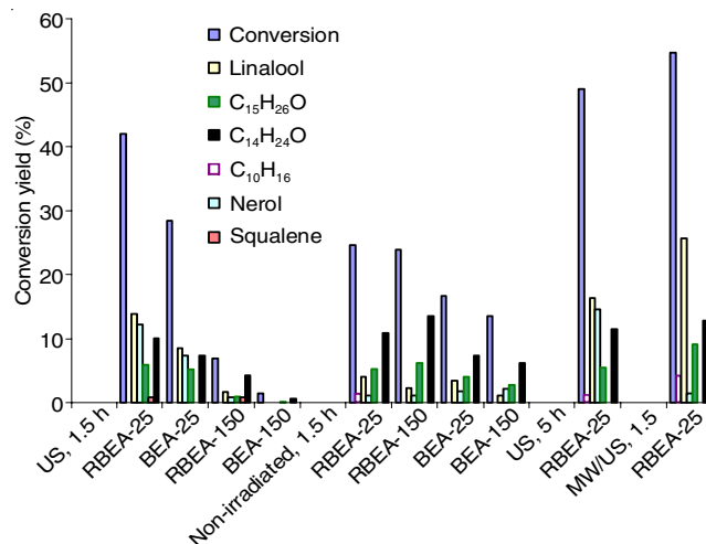
Fig. 9. Comparison of geraniol conversions and yields of products in reactions on beta-type zeolite catalysts. Reaction conditions: ultrasonic irradiation (350 W, 1.5 h; 5 h), without it (non-irradiated, 1.5 h) and simultaneous MW/US (550 W/300 W, 1.5 h) irradiation; catalyst loading – 0.92 mol of geraniol/g catalyst, argon atmosphere, run time – 1.5 h, 5.0 h, temperature – 80 °C
