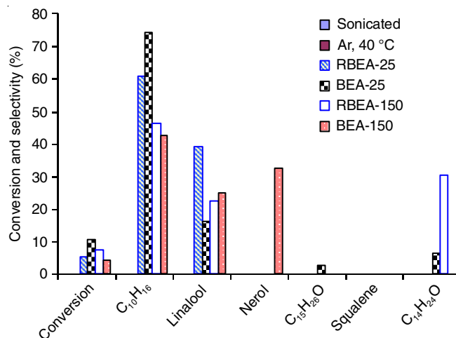
Fig. 3. Conversion of geraniol under US irradiation on microporous BEA-25, BEA-150 and micro-mesoporous RBEA-25, RBEA-150 zeolites, medium – Ar, catalyst loading – 0.92 mol of geraniol/g catalyst. US power – 350 W (UMR-300B), run time – 1.5 h, temperature 40 °C
