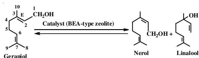
Scheme-I: Ultrasonically activated isomerization of geraniol into linalool and nerol
