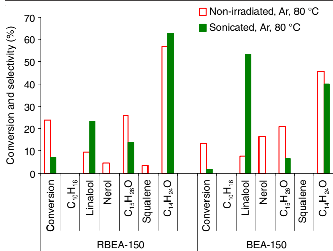
Fig. 4. Comparison of the conventional catalytic activity of zeolites (BEA-150 and RBEA-150) with activity in irradiated reaction of geraniol conversion; medium – US power –350 W (UMR-300B), Ar atmosphere, catalyst loading – 0.92 mol of geraniol/g catalyst, run time –1.5 h, temperature 80 °C
