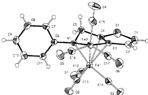
Fig. 1. Molecular structure of [ \mu_2 - \eta^3 -(Ph)N-CH 2 -C=C-C(H)=C(H)-S]Fe 2 (CO) 6 7.
