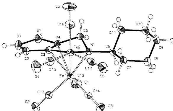
Fig. 2. Molecular structure of [\mu_2-\eta^3-(C_6H_{11})N-CH_2-\bar{C}\equiv C-C(H)=C(H)-S]Fe_2(CO)_6 8 .
