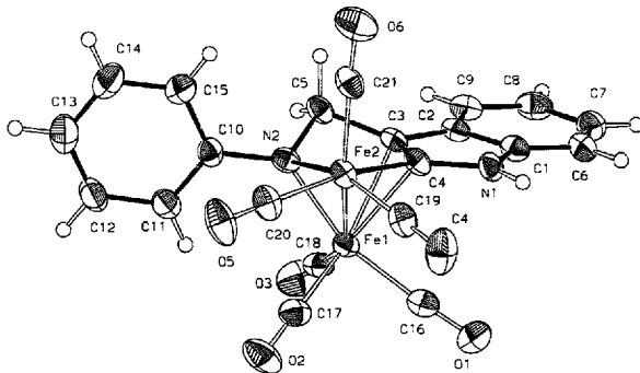
Fig. 6. Molecular structure of [\mu_2\text{-}\eta^3\text{-(Ph)N-CH}_2\text{-C}\equiv\text{C-N(H)-C(H)=C(H)-(CH}_3\text{)}]\text{Fe}_2(\text{CO})_6 19.
