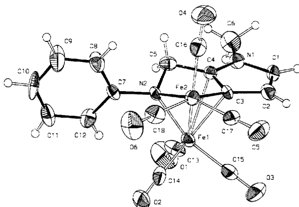
Fig. 3. Molecular structure of [\mu_2-\eta^3-(Ph)N-CH_2-\bar{C}\equiv C-C(H)=C(H)-NMe]Fe_2(CO)_6 10 .
