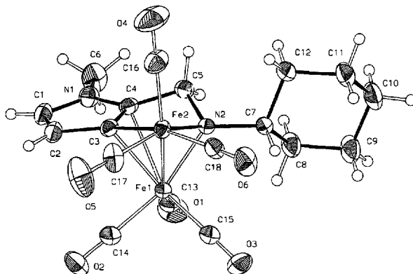
Fig. 4. Molecular structure of [\mu_2-\eta^3-(C_6H_{11})N-CH_2-\overline{C=C-C(H)=C(H)-NMe}]Fe_2(CO)_6 11.
