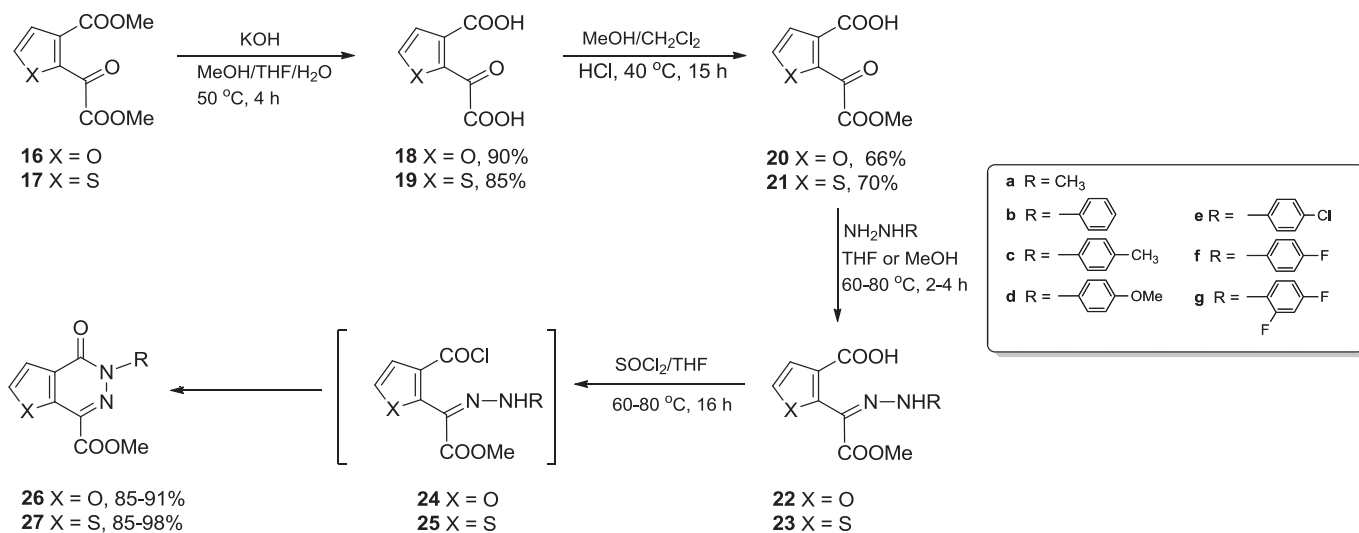
Scheme 3. Synthesis of furo- and thienocondensed pyridazinone derivatives.
