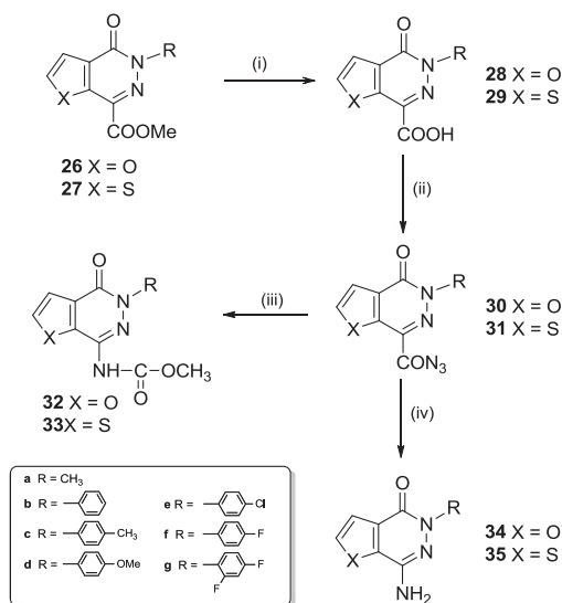
Scheme 4. Synthesis of furo- and thienocondensed aminopyridazinone derivatives. (i) KOH, CHCl 3 /THF/MeOH/H 2 O, 50 °C (57–78%); (ii) a: SOCl 2 , CHCl 3 /MeCN reflux or (COCl) 2 , DMF, CH 2 Cl 2 , b: NaN 3 , acetone (62–95%); (iii) a: benzene, reflux b: MeOH (43–83%); (iv) a: benzene, reflux b: 8 M HCl c: 2 M NaOH (42–68%).
