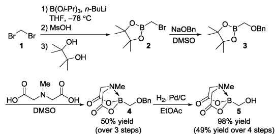
Scheme 1 Preparation of hydroxymethyl(MIDA)boronate.
