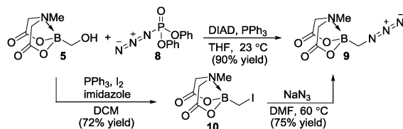
Scheme 2 Synthesis of azidomethyl(MIDA)boronate.
