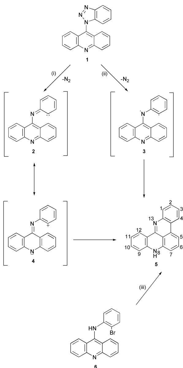
Scheme 1 Reagents and conditions: (i) h\nu , acetonitrile; (ii) heat, 259 °C; (iii) \text{Bu}_3\text{SnH} , AIBN, toluene, reflux.
