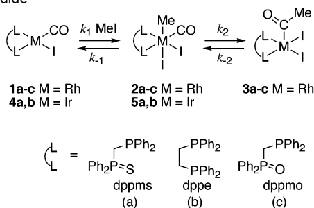
Scheme 3. General Scheme for Reactions of [\text{M}(\text{CO})(\text{L}-\text{L})\text{I}] with Methyl Iodide a
