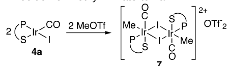
Scheme 5. Addition of Methyl Triflate to 4a
