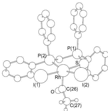
Figure 1. X-ray structure of [Rh(dppms)I 2 (COMe)] ( 3a ). Hydrogen atoms on the dppms ligand are omitted for clarity. Selected geometric data are given in Table 1.
