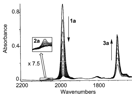
Figure 5. Series of IR spectra for the reaction of 1a with MeI (8 M in \text{CH}_2\text{Cl}_2 , 10 °C). Note the weak band due to intermediate 2a .
