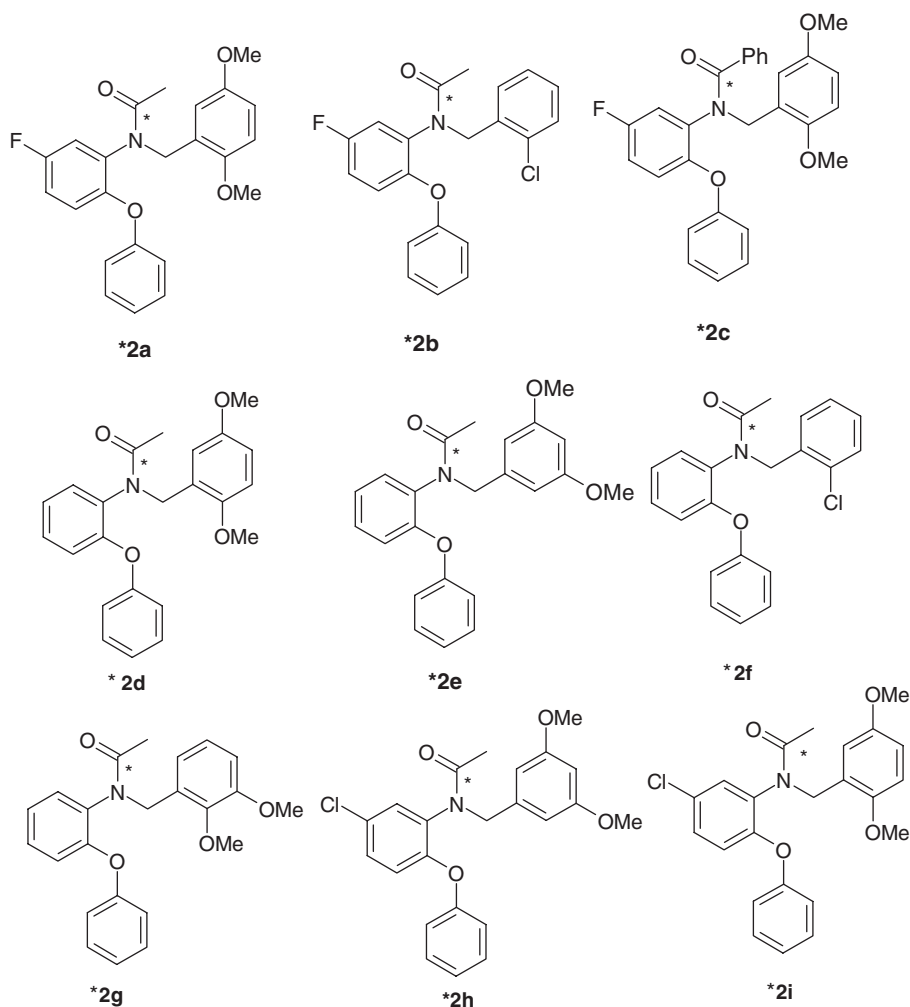
Figure 2 Target ^{11}\text{C} -labelled molecules, * = ^{11}\text{C} -labelled.
