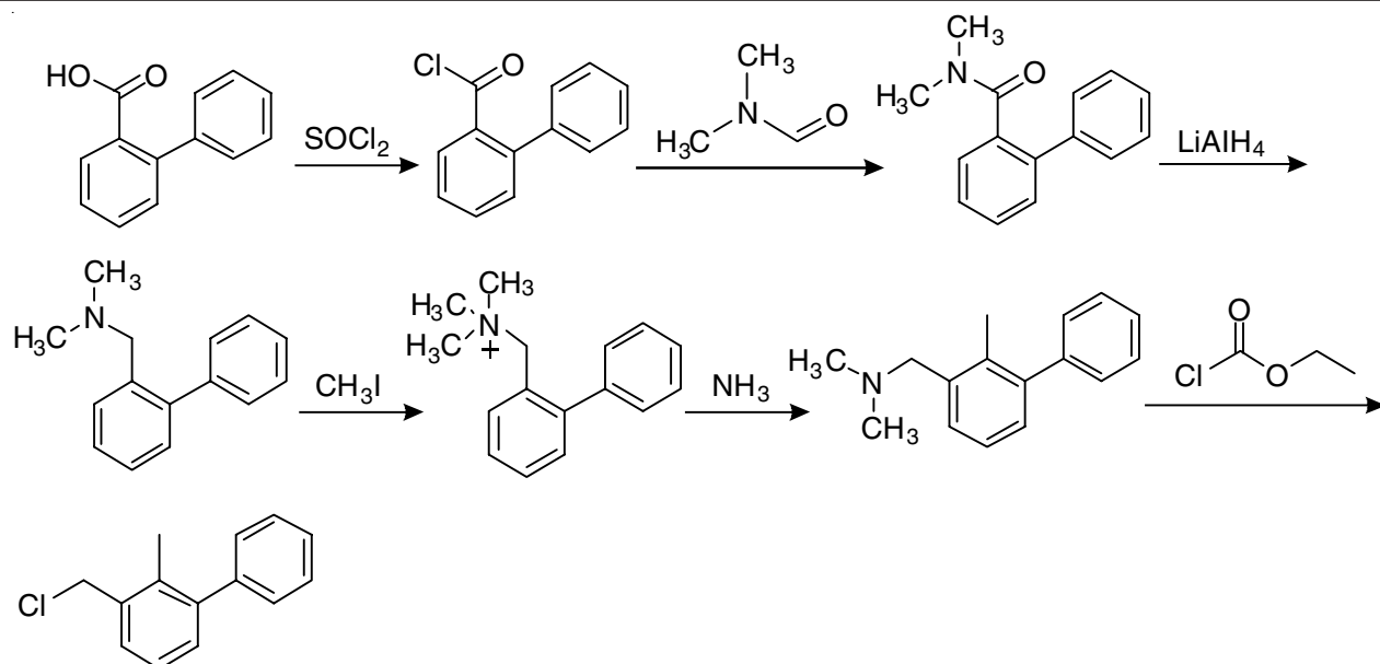
Scheme-I: Traditional synthetic process of 3-(chloromethyl)-2-methyl-1,1'-biphenyl from [1,1'-biphenyl]-2-carboxylic acid
