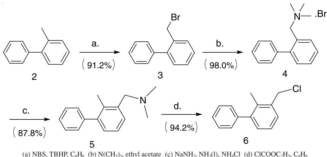
Scheme-II: Synthetic scheme of 3-(chloromethyl)-2-methyl-1,1'-biphenyl from 2-methyl-1,1'-biphenyl
