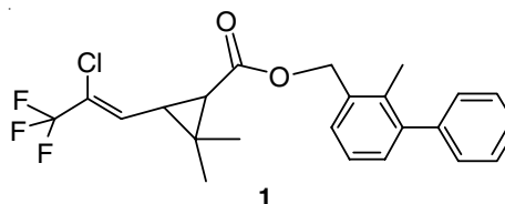
Fig. 1. Structure of bifenthrin
