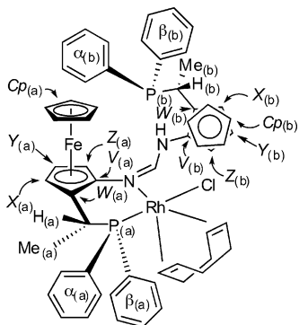
( κ-N,P -Bis[( S )-2-((1 R )-1-(diphenylphosphino)ethyl]ferrocen-1-yl]formamidinato)(chloro)(η 4 -1,4-cyclooctadiene)rhodium(I) (10)
