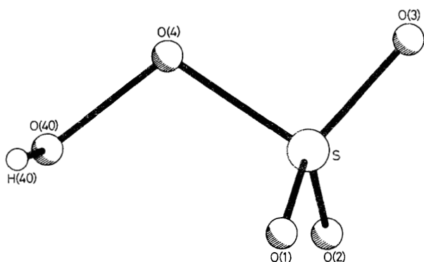
Figure 1. Structure of the \text{HSO}_5^- anion in (1). Bond lengths: S–O(1), 1.444(2); S–O(2), 1.437(2); S–O(3), 1.435(2); S–O(4), 1.632(2); O(4)–O(40), 1.460(3) Å. Bond angles: O(1)–S–O(2), 113.1(1); O(1)–S–O(3), 115.0(1); O(1)–S–O(4), 105.9(1); O(2)–S–O(3), 115.2(1); O(2)–S–O(4), 106.8(1); O(3)–S–O(4), 99.0(1); S–O(4)–O(40), 109.4(2)°.
