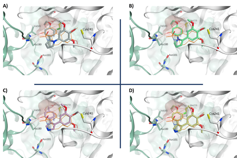
Fig. 3. Proposed binding modes for compounds 9o (A), 10h (B), 11c (C) and 11j (D) in the colchicine site. The trimethoxyphenyl ring is in proximity of \beta Cys241, while the differently substituted phenyl rings are placed in a hydrophobic sub-pocket formed near \beta Met259, \beta Thr314, \alpha Ala180 and \alpha Val181. The pyrrole nitrogen of 11c and 11j is oriented toward \alpha Asn101. Distance between the nitrogen atom (donor) of 11c and 11j to the oxygen atom (acceptor) of \alpha Asn101 is 3.39 and 3.41 Å respectively and thus in the range of a moderate-weak H-bond. Co-crystallized colchicine is shown in orange. The tubulin \alpha -subunit is shown as a mint green ribbon, while the \beta -(delete space) subunit is represented as a white ribbon. The hydrophobic sub-pocket is highlighted as a red surface. Hydrogen atoms of compounds are not shown to enhance the clarity of the Figure.
