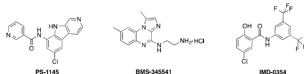
Figure 1: PS-1145, BMS-345541 and IMD-0354 as examples of IKKβ inhibitors.
