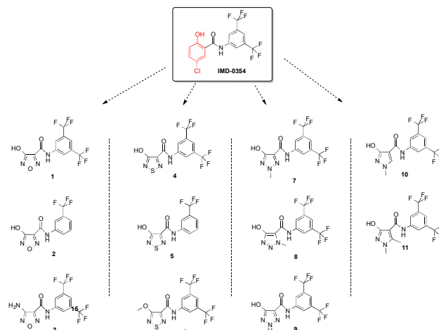
Figure 2: The bioisosteric scaffold hopping strategy applied to IMD-0354 using hydroxyoxadiazole , hydroxythiadiazole , hydroxytriazole and hydroxypyrazole scaffolds.
