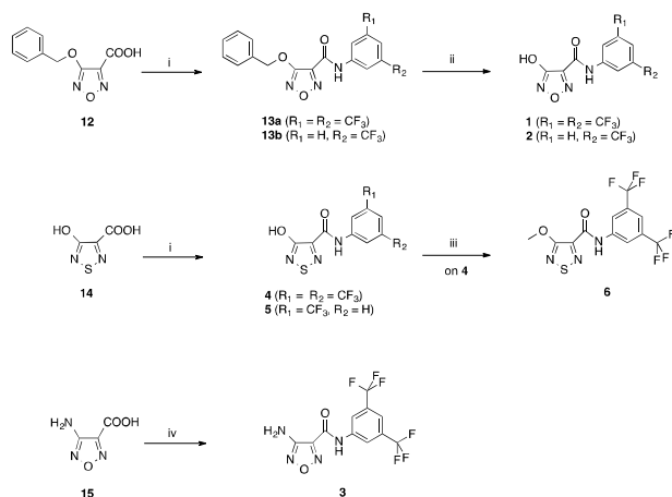
Scheme 1. Synthesis of 1,2,5-oxadiazole and thiadiazole analogues 1 - 6 : i) a) oxalyl chloride, DMF, dry THF, b) substituted aniline, dry pyridine, dry THF; ii) H 2 , Pd/C, dry THF; iii) CH 3 I, Cs 2 CO 3 , dry THF; iv) HBTU, DMAP, 3,5-bis(trifluoromethyl)aniline, dry DMF.
