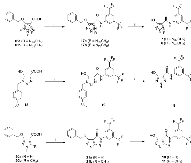
Scheme 2. Synthesis of triazole and pyrazole analogues ( 7 - 11 ): i) a) oxalyl chloride, DMF, dry THF; b) 3,5-bis(trifluoromethyl)aniline, dry pyridine, dry THF; ii) H 2 , Pd/C, dry THF; iii) TFA, 45°C.
